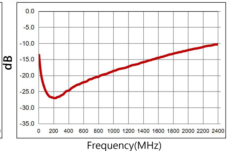
Isolation(pin4-3)
