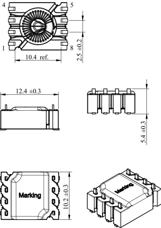
Cosmetic Dimension
